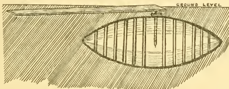
TORPEDO - MORRIS ISLAND.
